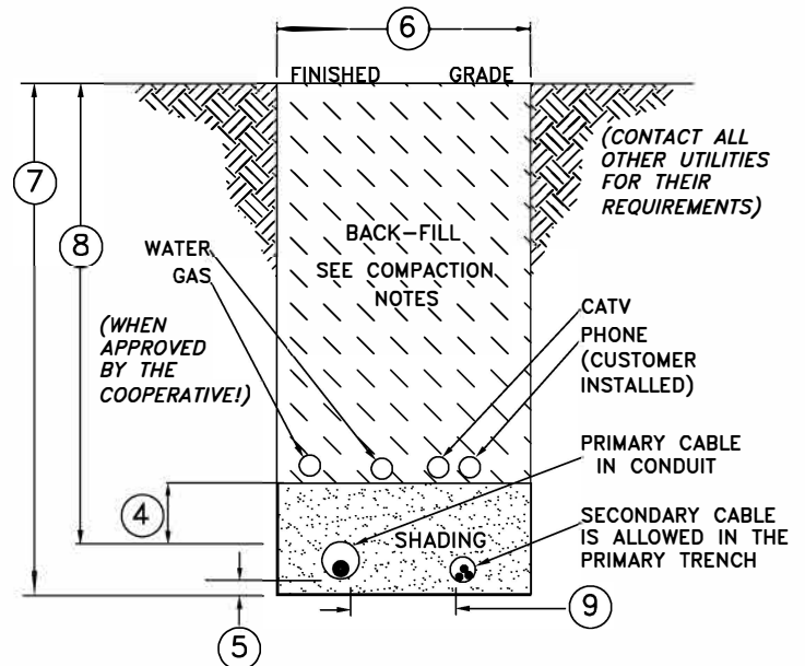
MAIN TRENCH DETAIL, UR2-54
