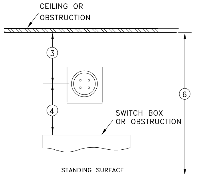
VERTICAL CLEARANCE
