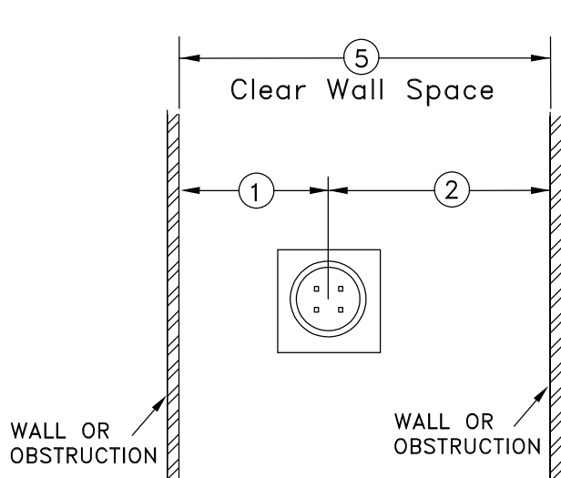
HORIZONTAL CLEARANCE
