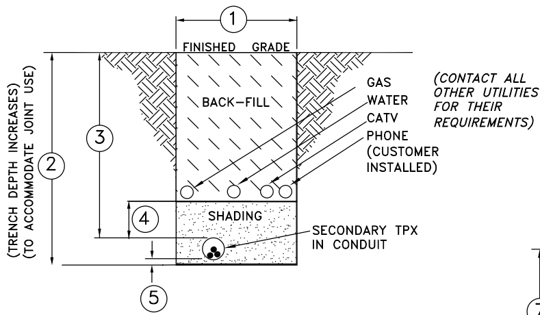
SECONDARY TRENCH DETAIL, UR2-32
