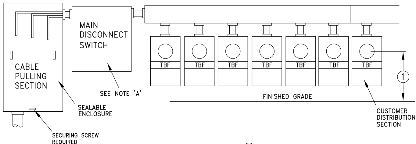
Figure 10-2 Commercial Ganged Meter Socket Installation
