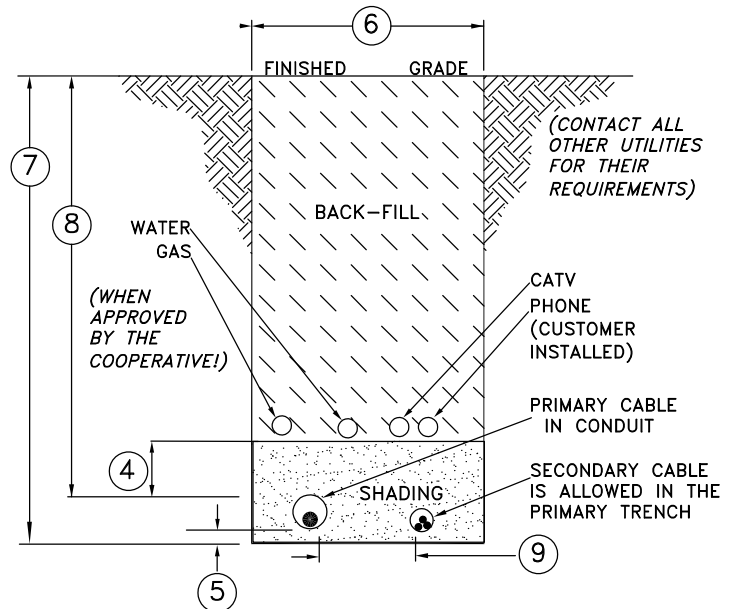
MAIN TRENCH DETAIL, UR2-54
