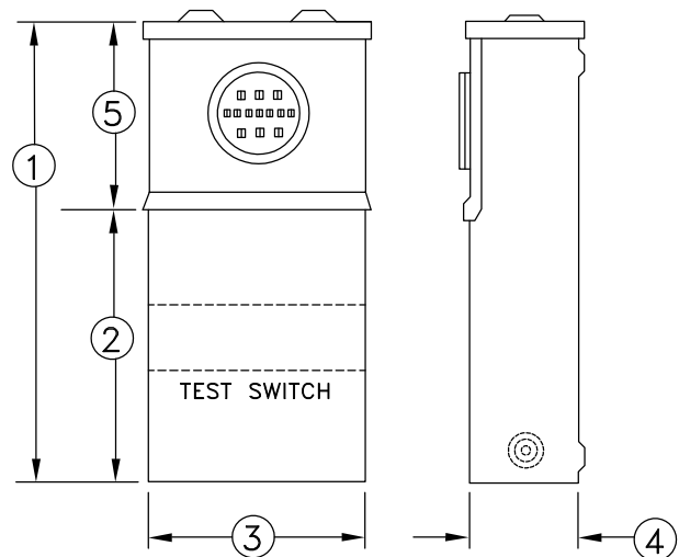
THREE PHASE – 13 JAW
